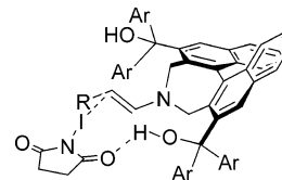
Figure 1. Transition state model for the direct asymmetric iodination reaction catalyzed by (S)-1d.
