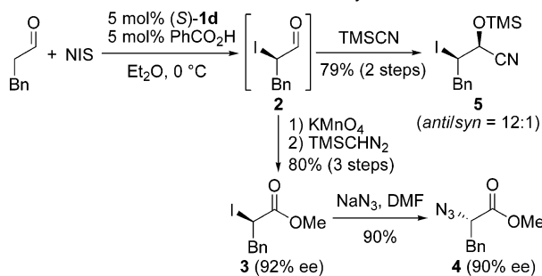
Scheme 2. Transformation of \alpha -Iodoaldehyde
